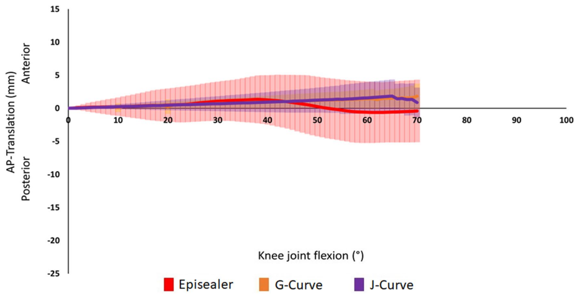
Fig. 11 Relative kinematics during loaded lunge at the medial condyle. Comparison between episealer and TKA knees
